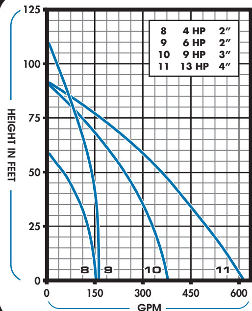
SPE AL and FSP AL PERFORMANCE CURVES TRASH HANDLING APPLICATIONS
