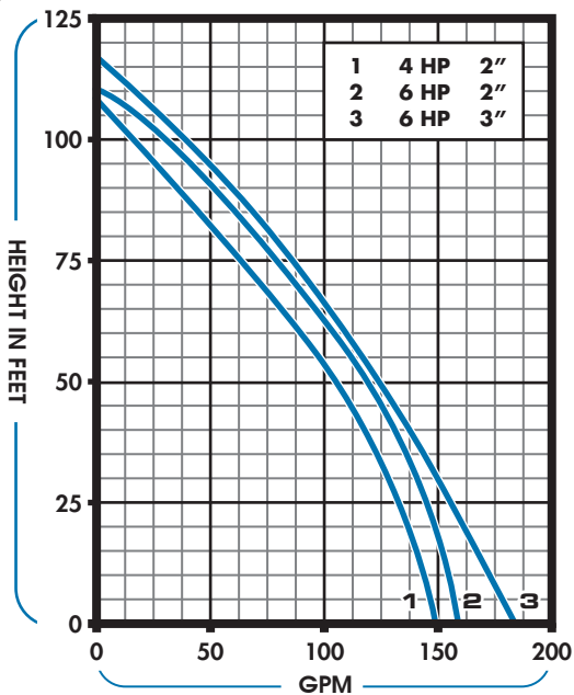
SPE AL and FSP AL PERFORMANCE CURVES GENERAL PURPOSE
