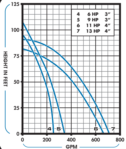
SPE AL and FSP AL PERFORMANCE CURVES PROFESSIONAL & COMMERCIAL
